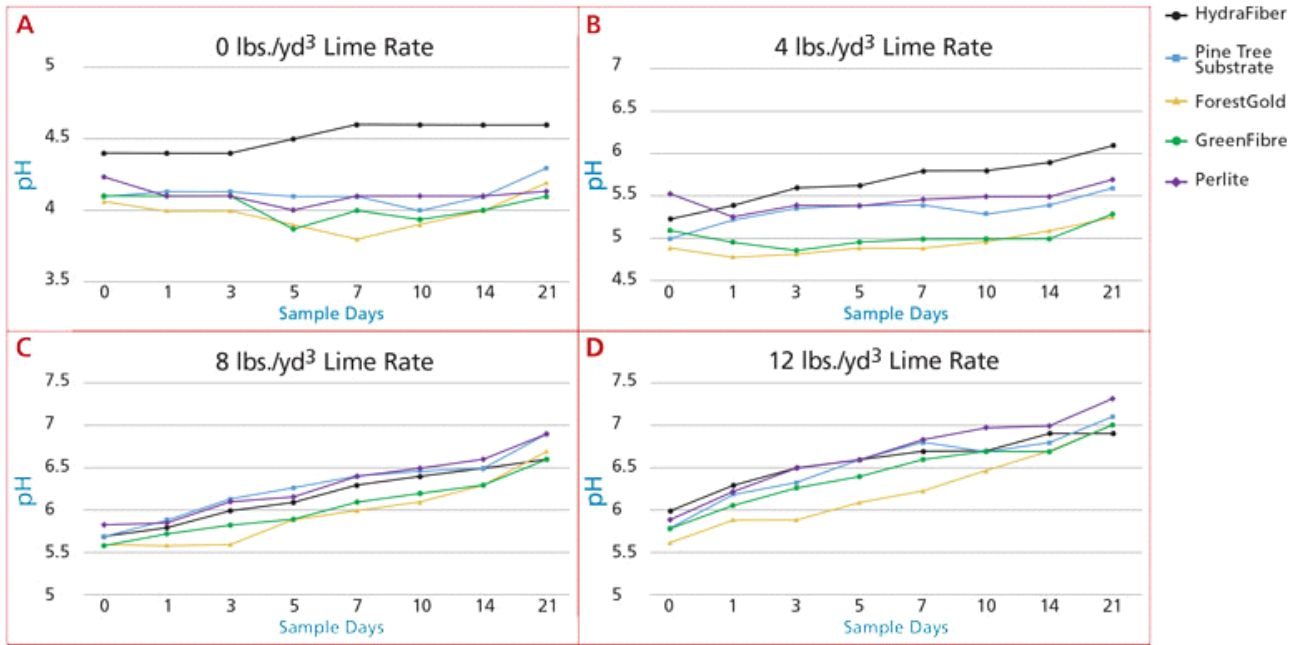
Figure 2: Substrate pH of peat moss amended with 40% (by volume) of either perlite or four commercial wood products when limed at 0, 4, 8 or 12 lbs./yd 3 .
