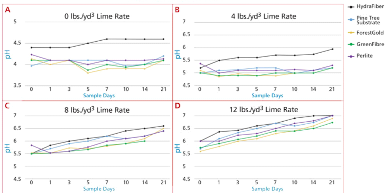
Figure 1: Substrate pH of peat moss amended with 20% (by volume) of either perlite or four commercial wood products when limed at 0, 4, 8 or 12 lbs./yd³.
